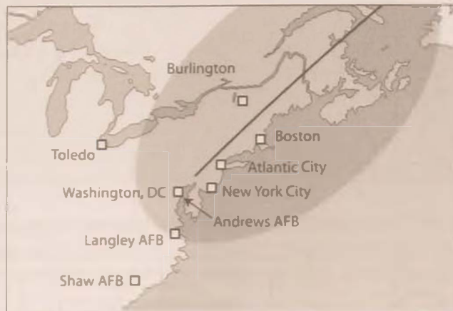
Exoatmospheric intercepts; time of flight not limited (earliest launch: 1,312 seconds)
